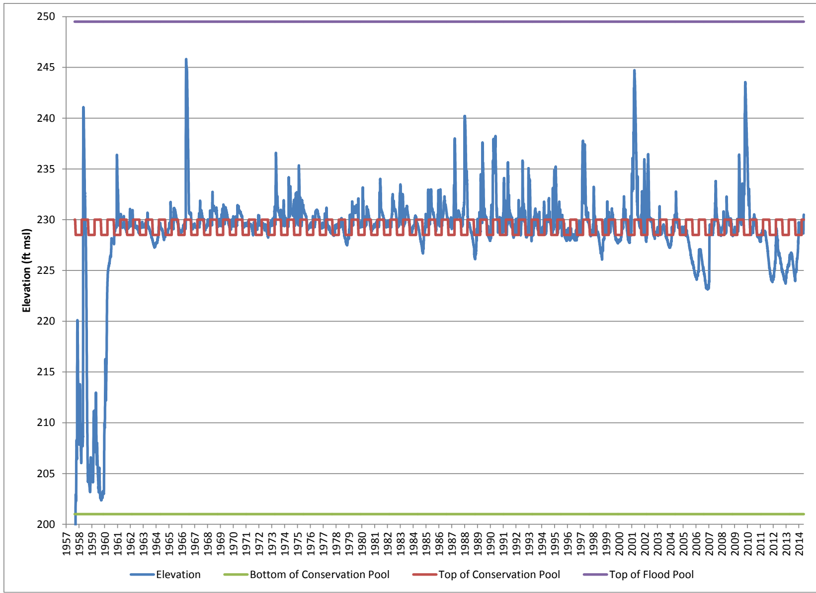
Figure 2 Lake O' the Pines Historical Elevations
