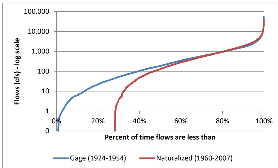
Figure 7 Cumulative Frequency of gage flows for Pre-LOTP period (1924-1954) and synthetic naturalized flows for Post – LOTP period (1960-2007)
